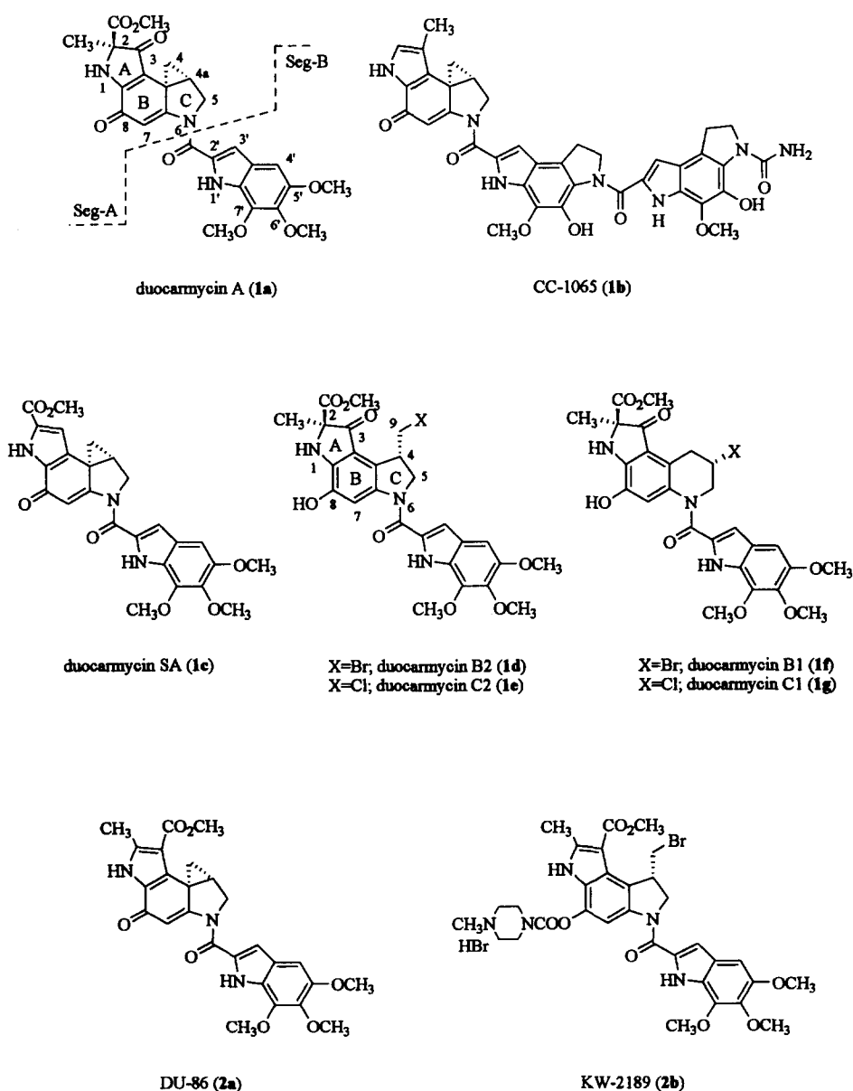
Figure 1. Structures of duocarmycins, CC-1065 and duocarmycin derivatives.
