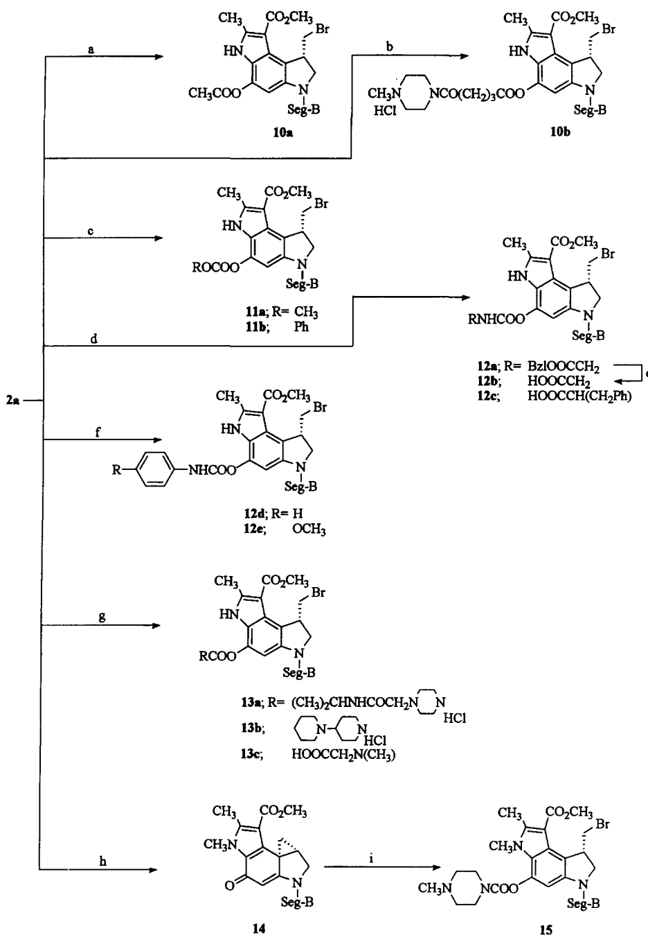
Scheme 2. (a) HBr, CH 3 CN, then Ac 2 O, 4-(dimethylamino)pyridine (DMAP), CH 2 Cl 2 ; (b) HBr, CH 3 CN, then 4-(4-methyl-1-piperazinyl)butyric acid, DMAP, dicyclohexylcarbodiimide (DCC), CH 2 Cl 2 , then HCl, EtOH; (c) HBr, CH 3 CN, then CH 3 OCOC or PhOCOC, Et 3 N, CH 2 Cl 2 ; (d) HBr, CH 3 CN, then 4-nitrophenyl chloroformate, Et 3 N, CH 2 Cl 2 , then glycine benzylester TsOH or phenylalanine; (e) H 2 , 10% Pd/C; (f) HBr, CH 3 CN, then phenyl isocyanate or 4-methoxyphenyl isocyanate; (g) HBr, CH 3 CN, then 4-nitrophenyl chloroformate, Et 3 N, CH 2 Cl 2 , then N -isopropyl-1-piperazineacetamide or 4-piperidinopiperidine or sarcosine, then HCl, EtOH; (h) CH 3 I, K 2 CO 3 , DMF; (i) HBr, CH 3 CN, then 4-nitrophenyl chloroformate, Et 3 N, CH 2 Cl 2 , then N -methylpiperazine.
