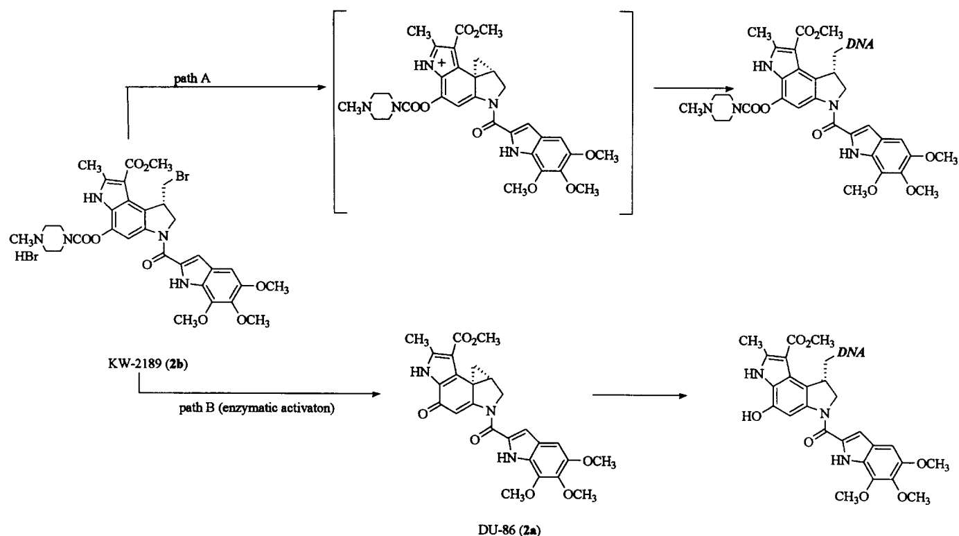
Figure 2. Mechanism of alkylation for DNA of 2b (KW-2189).
